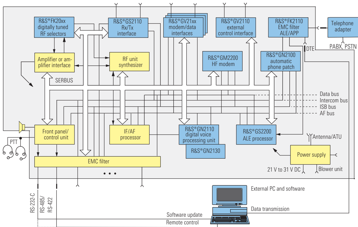
Block diagram of the R&S® XK2100 and R&S® GX2900: the base units of the R&S® Series 2000 systems are equipped with six standard modules and provide spare slots for options (blue). Software updates are conveniently performed from a PC via the RS-232-C interface.
