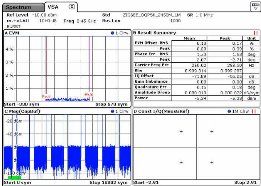
Figure 7 FSV-K70 result screens: Evaluation Range indicated by vertical lines in the EVM plot and red double bars in the headlines of the Result Summary and the Constellation diagram
