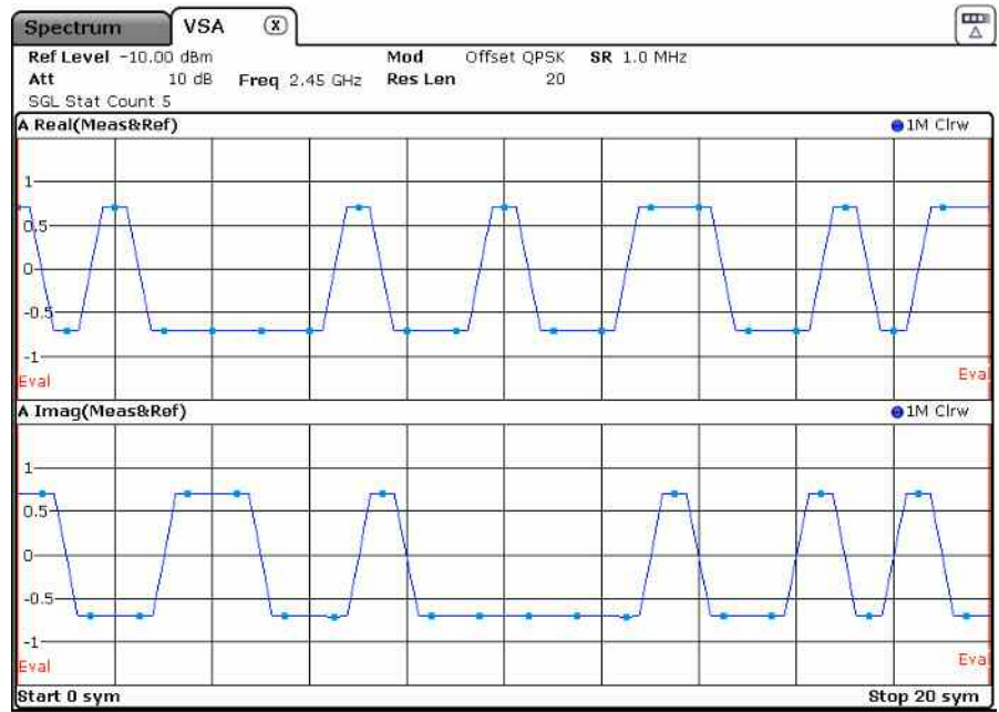
Figure 3 For OQPSK I and Q transitions never occur at the same time instance. This limits the maximum phase change to 90° and reduces amplitude variations
