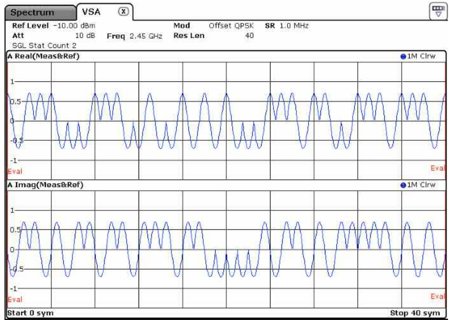
Figure 4 I and Q display for OQPSK after pulse shaping
