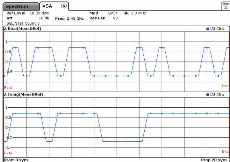
Figure 2 For QPSK, I and Q transitions occur at the same time instance. A simultaneous change is equivalent to a 180^\circ phase shift
