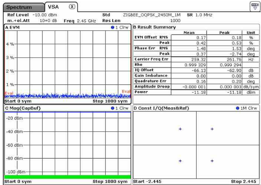
Figure 9 The EVM measurements with the R&S FSQ or R&S FSV shows a residual EVM of approx. 0.2%. This is a prerequisite for accurate EVM measurements
