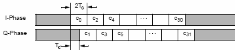
Figure 1 Timing offset as defined in IEEE std 802.15.4
