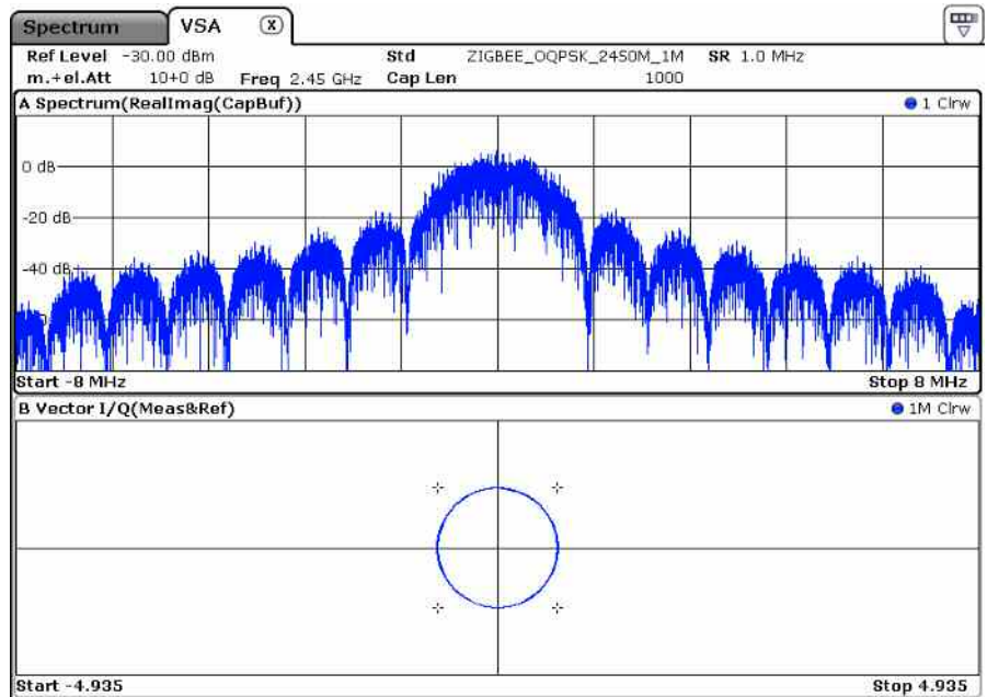
Figure 5 The vector diagram of the half-sine filtered OQPSK shows a constant envelope
