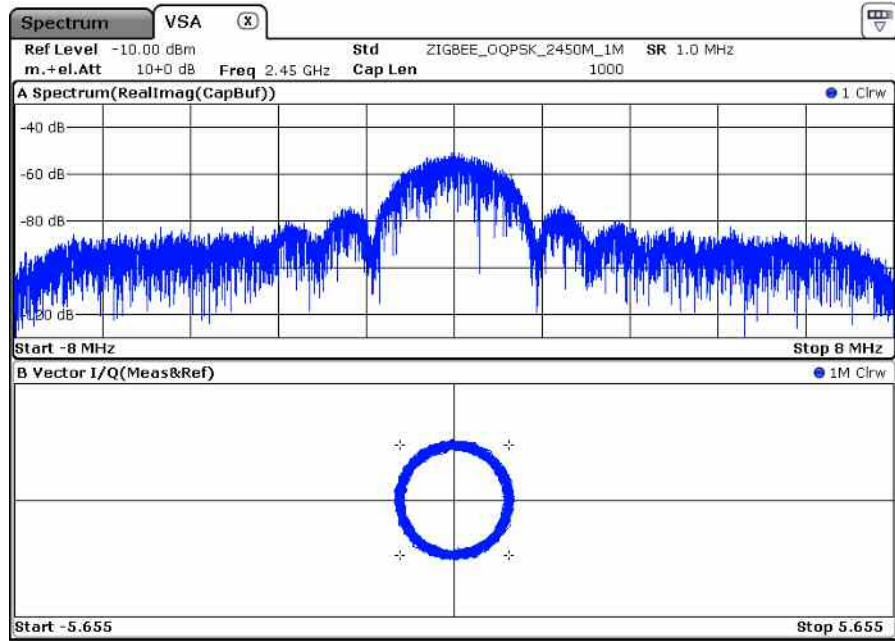
Figure 8 Weak ZigBee signal resulting in low S/N
