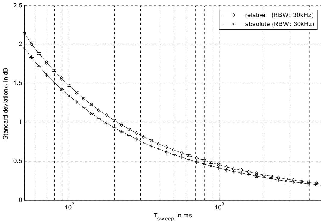
Standard deviation \sigma of spectrum emission mask measurement as a function of sweep time ( T_{sweep} )
