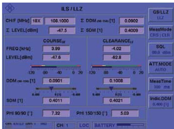
Simultaneous analysis of course and clearance signals.
