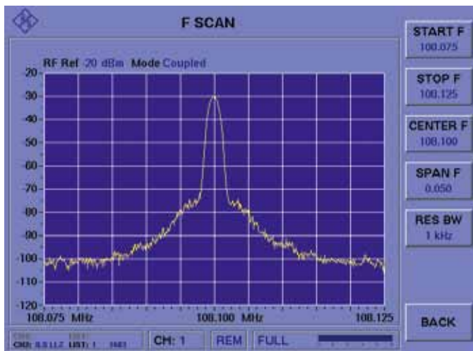
Spectrum analysis of the RF signal.
