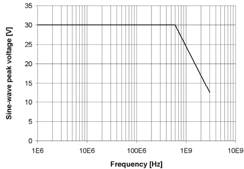
Non-destructive sine-wave peak voltage versus frequency.
