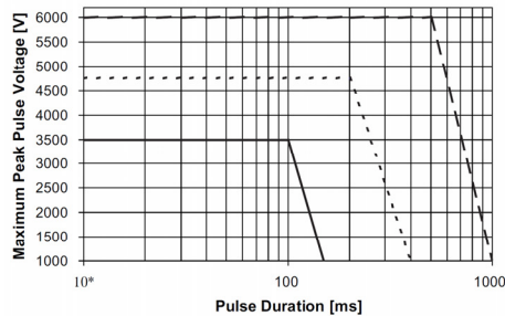
R&S®RT-ZH10/-ZH11 maximum pulse derating, CAT I.
