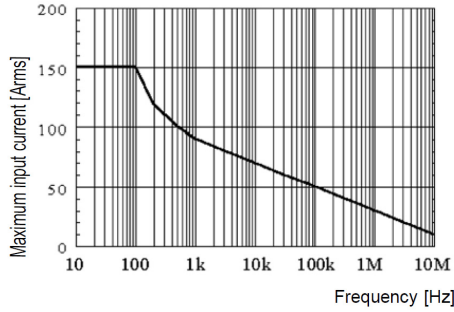
R&S®RT-ZC10 continuous maximum input current.
