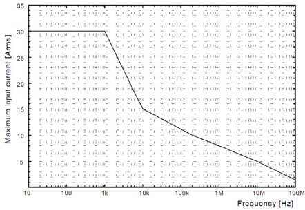
R&S®RT-ZC20 continuous maximum input current.
