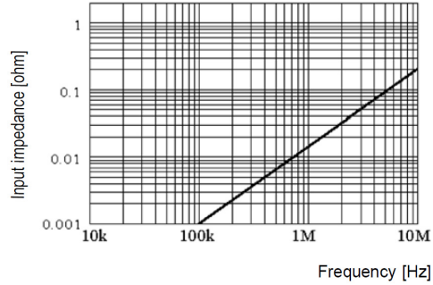
R&S®RT-ZC10 insertion impedance (meas.).
