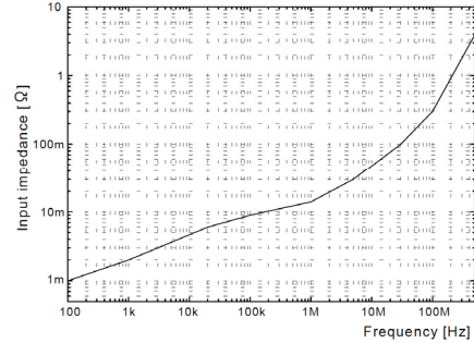
R&S®RT-ZC20 insertion impedance (meas.).
