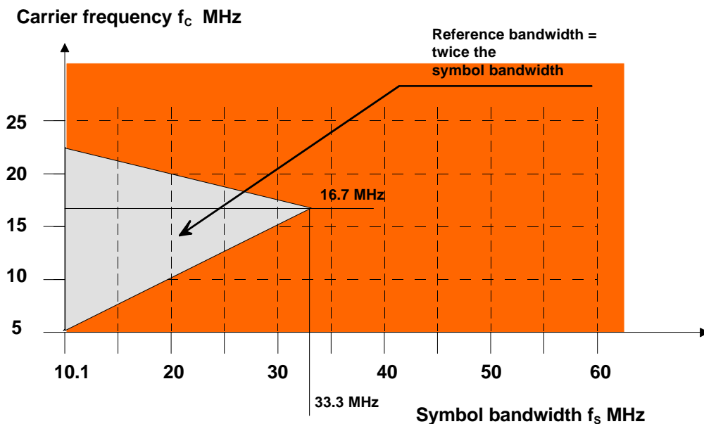
Fig. 11 Carrier frequency 5 \text{ MHz} < f_c < 22.5 \text{ MHz} as a function of symbol bandwidth f_s \geq 10.1 \text{ MHz}
