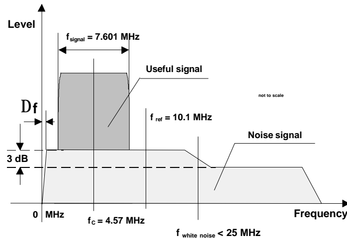
Fig. 13 Signal bandwidth f_{\text{signal}} as a function of f_c < 15 MHz for white noise
