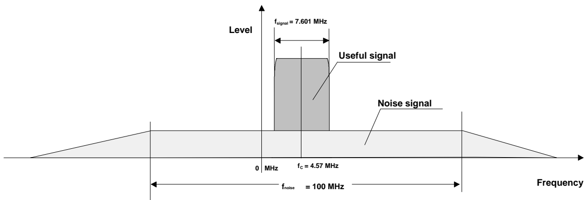
Fig. 8 Non-physical spectrum and broadband noise spectrum
