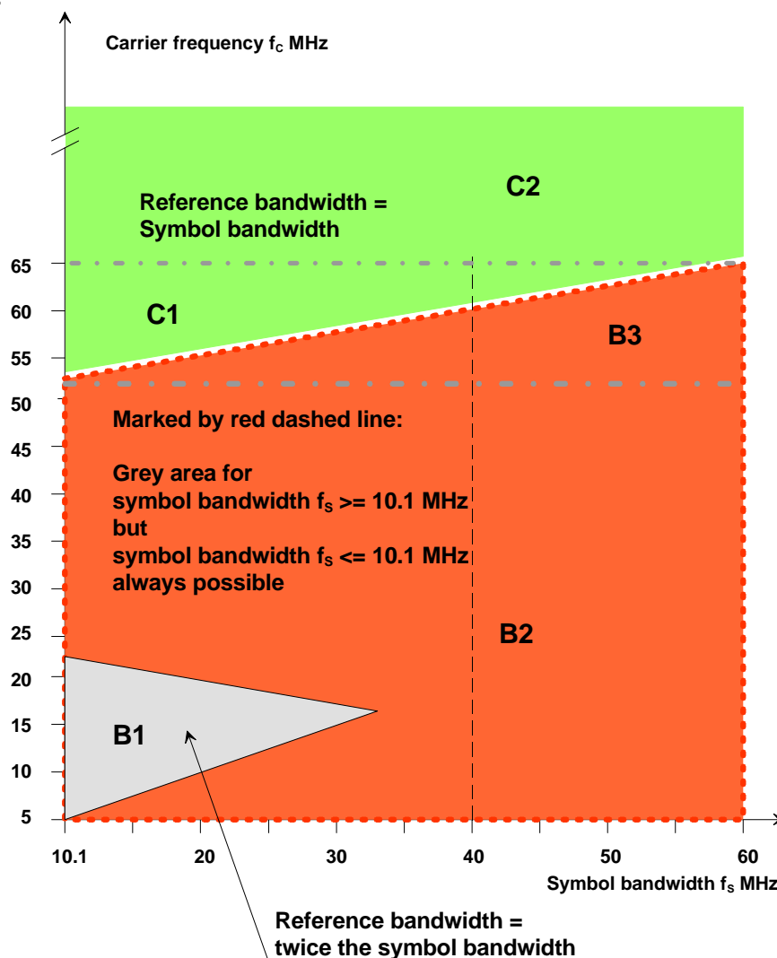
Fig. 12 Ranges B and C: f_c as a function of f_s \geq 10.1 \text{ MHz} or of the C/N reference bandwidth for white noise with correct C/N display on SFQ
