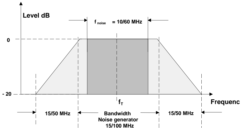
Fig. 2 Spectra of SFQ noise generator
