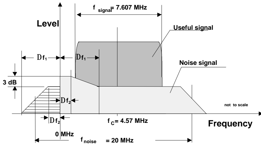
Fig 6 Real spectrum with noise reflection
