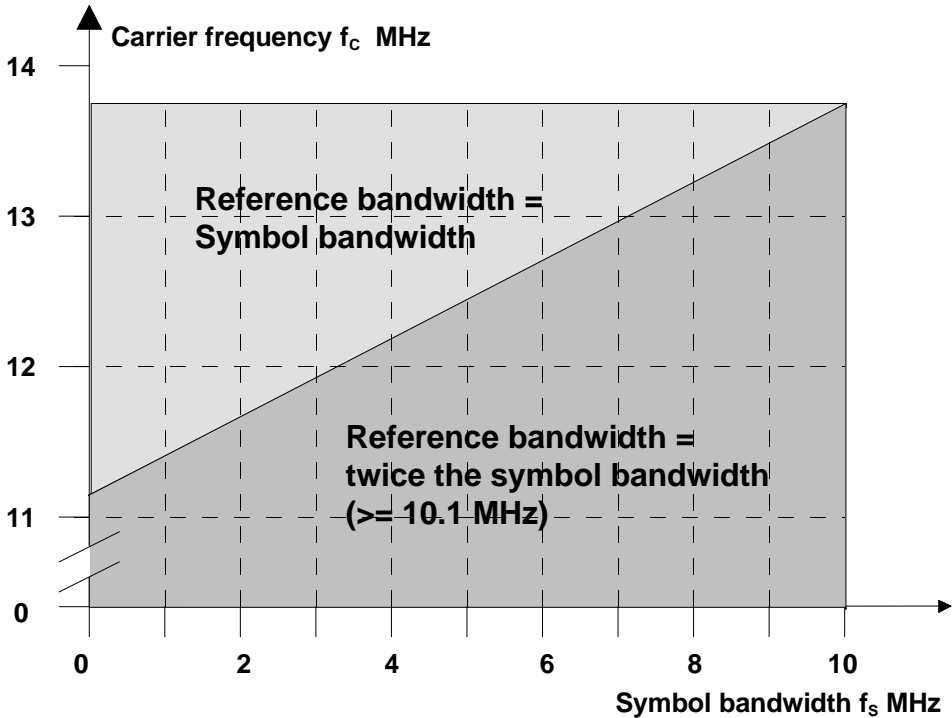
Fig. 10 Carrier frequency f_c < 15 MHz as a function of symbol bandwidth f_s \leq 10.0 MHz or C/N reference bandwidth for white noise and correct C/N display on the SFQ
