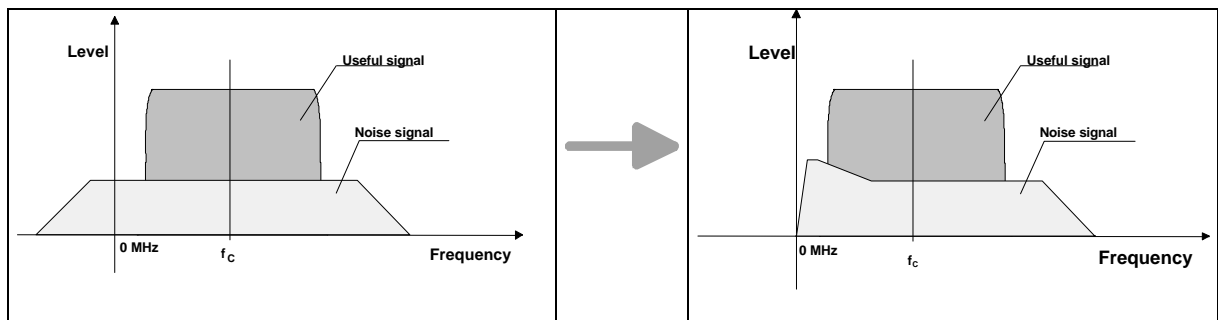
Fig. 3 Frequency reflection about 0 Hz
