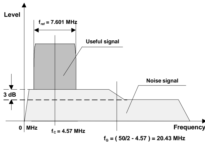
Fig. 9 Real spectrum and broadband noise spectrum
