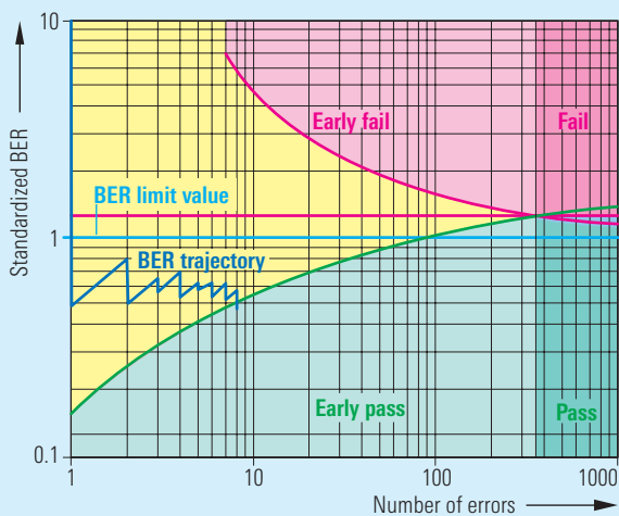
FIG 3 A time-independent evaluation diagram is used in practice. The BER standardized to the limit value is indicated vertically, and the bit and block errors are counted horizontally. The dark blue trace (BER trajectory) shows the evaluation process. As long as no new errors occur, the BER decreases constantly. If a new bit error occurs, the trace will extend by one error horizontally. At the same time, the BER deteriorates because of this error. This method is applied until the trace leaves the yellow area; measurement is then terminated and, depending on the location of the end point of the trace, the receiver BER – at a specified probability – is either better or worse than the limit value.
