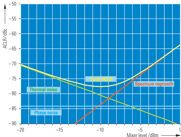
FIG 3 ACLR for a WCDMA signal (3.84 MHz bandwidth, 12 dB crest factor)
