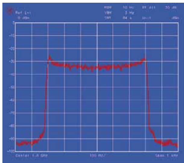
Fig. 7: Rayleigh fading (Doppler spectrum), generated at a speed of 180 km/h (RF = 1.8 GHz)
